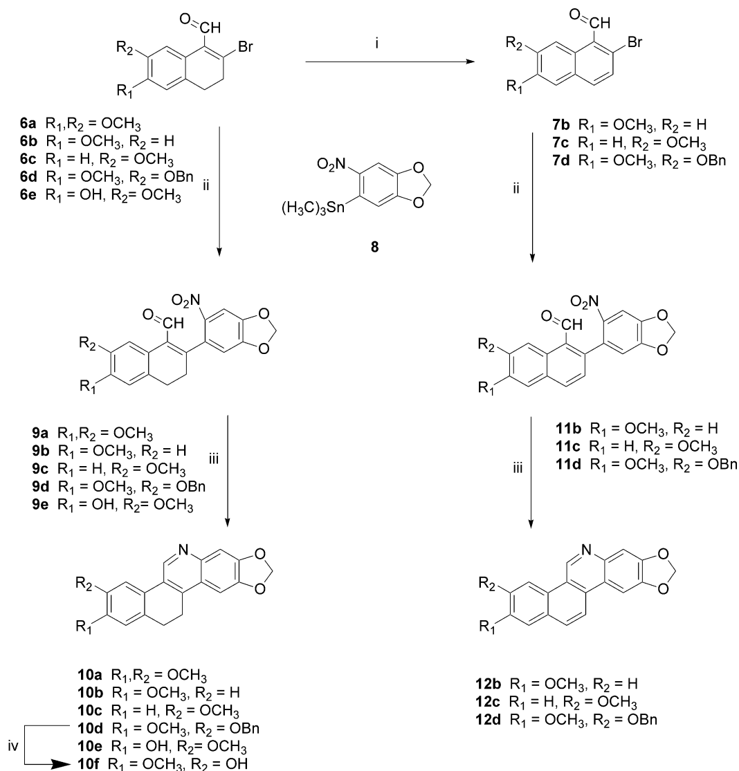
Scheme 1. Synthetic approach to the preparation of 8,9-methylenedioxybenzo[ l ]phenanthridine derivatives, 10a–10f and 12b–12d : (i) DDQ, toluene; (ii) \text{Pd}(\text{PPh}_3)_4 , CuBr, THF, reflux; (iii) Zn dust, AcOH, reflux; (iv) \text{Ra-Ni} , \text{H}_2 at 44 psi.
