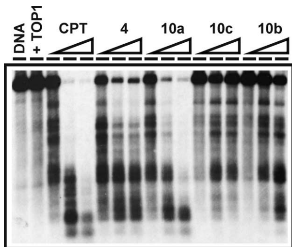
Figure 2. Stimulation of enzyme-mediated DNA cleavage by camptothecin (CPT), 4 , 10a , 10c , and 10b using human TOP1. The first lane is DNA control without enzyme. The second lane is the control with enzyme alone. The rest of the lanes contain human TOP1 and serially (10-fold each) diluted compounds from 0.01 to 1.0 \mu\text{M} for CPT and 1.0 to 100 for compounds 4 , 10a , 10b and 10c .
